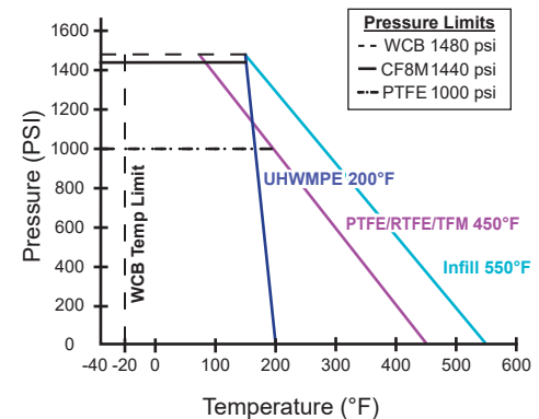
334F/S Pressure/Temperature Chart
